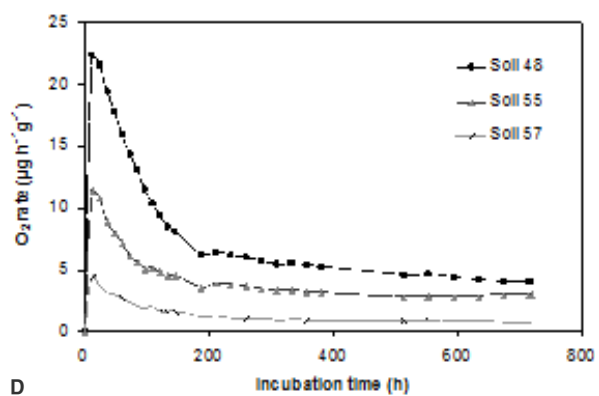
Figure 1. Cumulative O 2 consumption (A, C) and O 2 consumption rates (B, D) over 30 days of incubation for soils amended (top plots, A and B) and non-amended (bottom plots C and D) with sewage sludge.
